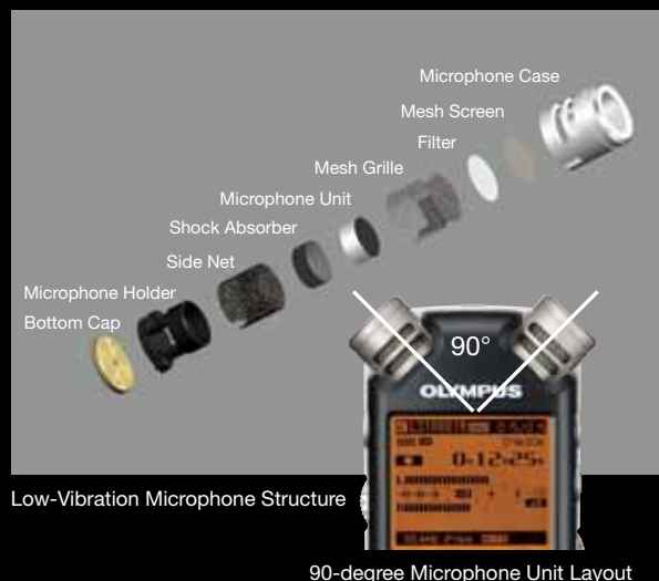
90-degree Microphone Unit Layout
